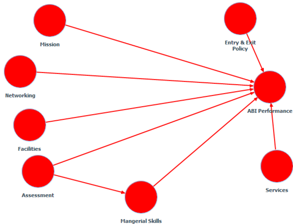
Figure 1: Proposed Model
